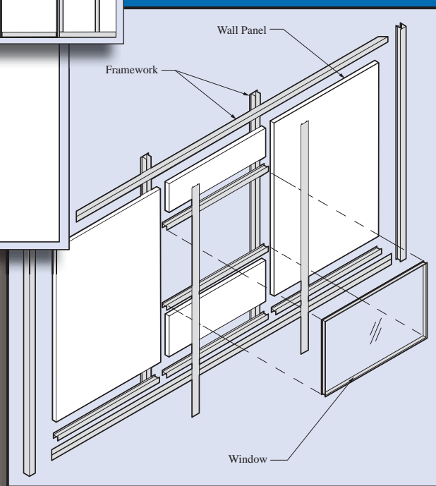
Exploded Wall Elevation View w/Window
