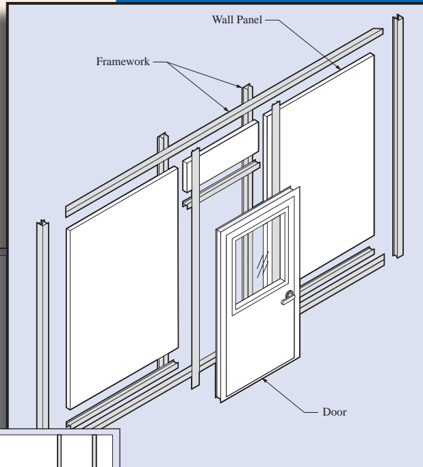
Exploded Wall Elevation View w/Entry Door
