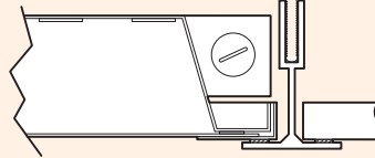
CRI 2" Walkable Grid 24 1/2" x 48 1/2" o.c.
