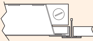
CRI 1 1/2" Cleanroom Grid 24" x 48" o.c.
