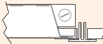
CRI 2" HD Structural Grid 24 1/2" x 48 1/2" o.c.
