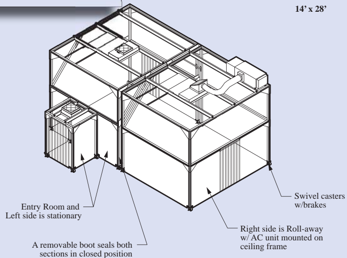
14' x 28'
