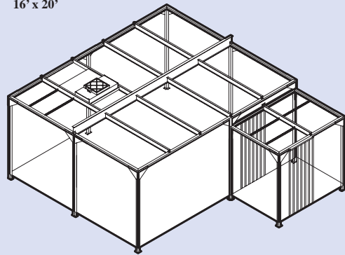
16' x 20'
