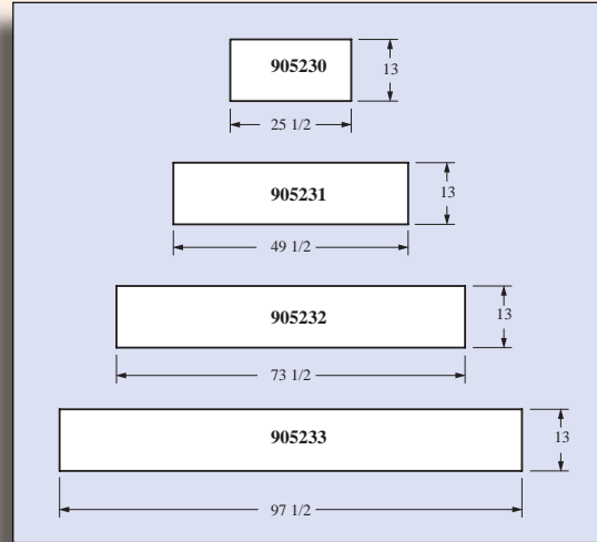
Face Shield Dimensions
