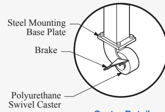
Caster Detail
