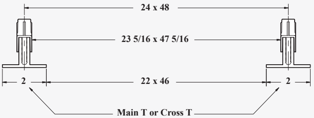
Undersize 24" x 48" o.c.
