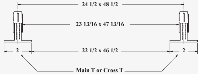
Standard 24 1/2" x 48 1/2" o.c.
