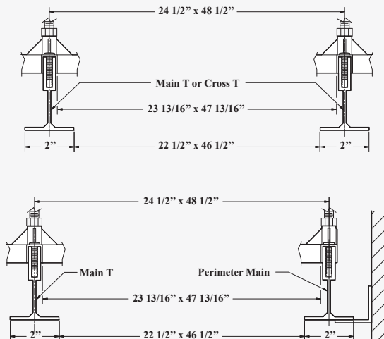
Standard 24 1/2" x 48 1/2" Centerline Spacing
