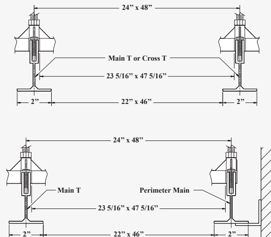
Undersize 24" x 48" Centerline Spacing
