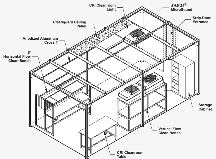
Typical Flexible Solutions Softwall Cleanroom by Clean Rooms International
