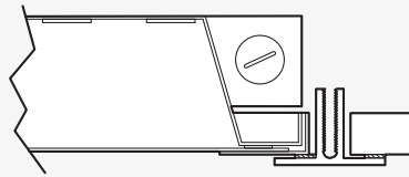
CRI 2" HD Structural Grid 24 1/2" x 48 1/2" o.c.
