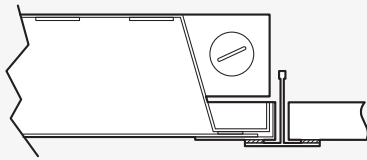
CRI 1 1/2" Cleanroom Grid 24" x 48" o.c.
