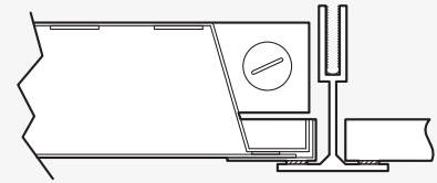
CRI 2" Walkable Grid 24 1/2" x 48 1/2" o.c.
