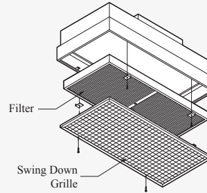
Exploded View
