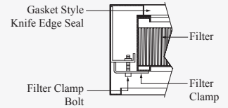
Filter Clamp Detail: CRF
